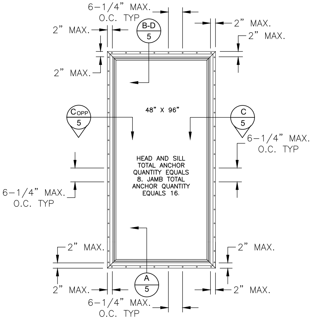
ANCHOR LAYOUT NAILING FIN INSTALLATION
