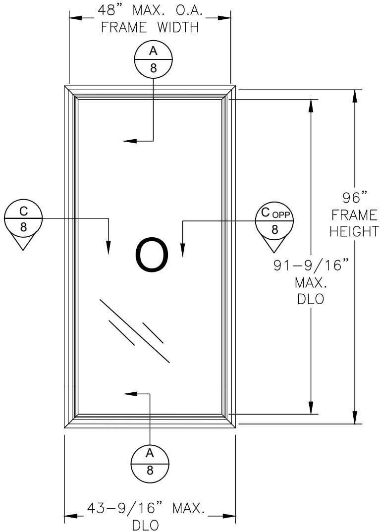
ELEVATION LAYOUT PICTURE WINDOW NAILING FIN FRAME
