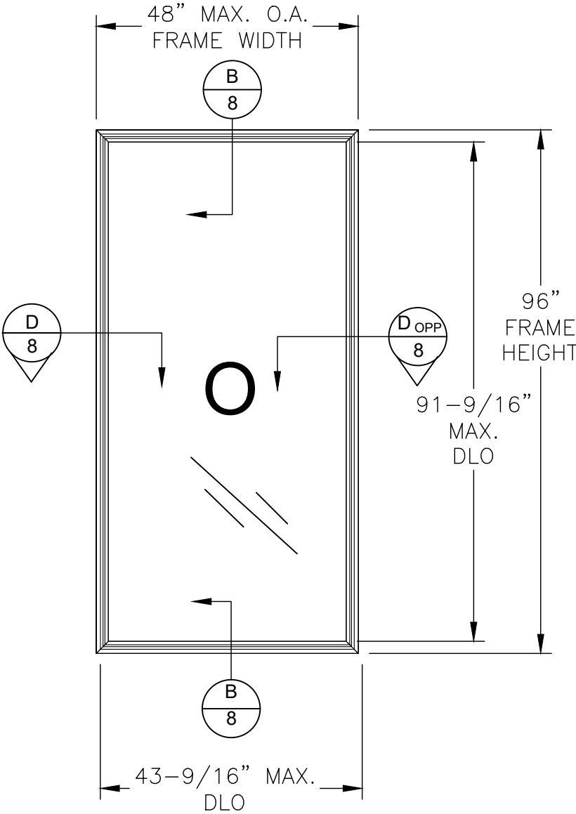
ELEVATION LAYOUT PICTURE WINDOW EQUAL LEG FRAME
