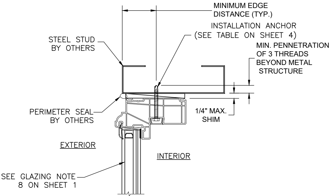
D 6 VERTICAL SECTION STEEL STUD STRUCTURE FRAME INSTALLATION HEAD SHOWN, SILL & JAMBS SIMILAR
