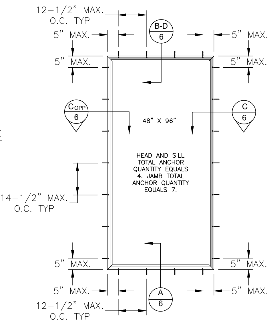
ANCHOR LAYOUT FRAME INSTALLATION
