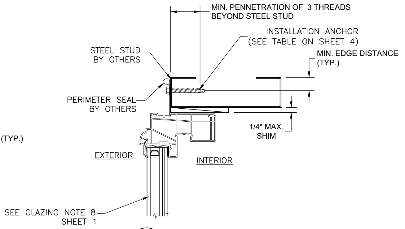
D 5 VERTICAL SECTION STEEL STUD STRUCTURE NAIL FIN INSTALLATION HEAD SHOWN, SILL & JAMBS SIMILAR
